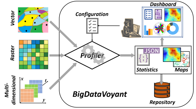
Figure 1: Processing flow for automated geodata profiling.
