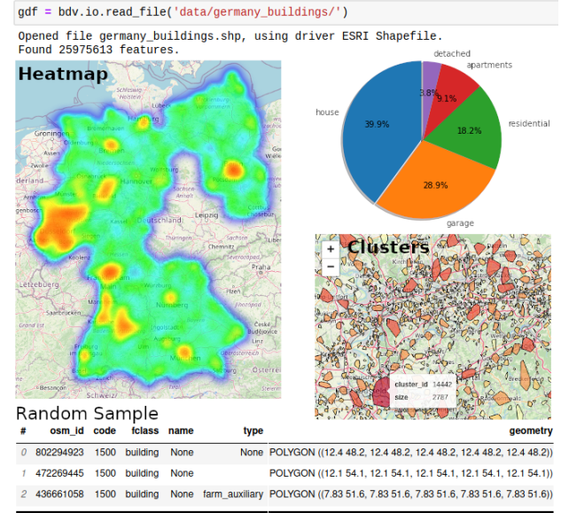
Figure 2: Visualization of automated metadata profiling a vector dataset of 25 million polygons (buildings in Germany) extracted from OpenStreetMap.
